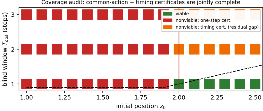
Figure 3: Whole-window hold-class coverage of Table 2: green = viable; red = nonviable under either class, diagnosed by the discrete one-step test; orange = nonviable only in the audited hold class , established by the discrete hold-class survival calculation. With per-step alternating actions, the orange cells are viable. The dashed curve is the hold-class boundary z_0 = 1 + T_{\text{obs}} , not an unrestricted boundary; the solid vertical line marks the one-step boundary z_0 = 2 .
